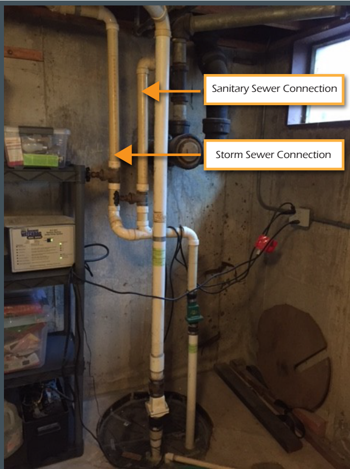
Illegal combination sump pump setup; servicing sanitary and storm water.
